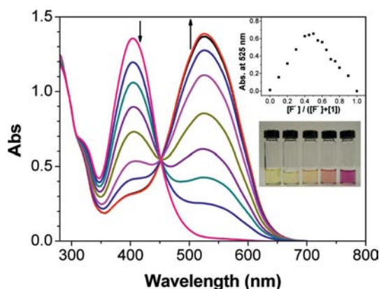
Figure 5. UV/Vis spectral changes of a DMSO solution of 1 ( 4.0 \times 10^{-5} \text{ mol L}^{-1} ) upon addition of a solution of (\text{Bu}_4\text{N})\text{F} ( 1.0 \times 10^{-2} \text{ mol L}^{-1} ). The inset shows the Job plot for the binding of 1 to \text{F}^- monitored at 525 nm ( [\text{F}^-] + [\text{1}] = 4.0 \times 10^{-5} \text{ mol L}^{-1} ) and the color change of DMSO solutions of 1 upon addition of (from left to right) 0, 0.25, 0.5, 0.75, and 1.0 equiv. \text{F}^- .
