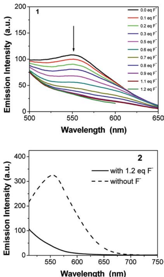
Figure 7. Changes in the emission spectra of 1 and 2 in DMSO solution ( 4.0 \times 10^{-5} \text{ mol L}^{-1} ) upon addition of (\text{Bu}_4\text{N})\text{F} ( \lambda_{\text{ex}} = 404 \text{ nm} for 1 and 430 \text{ nm} for 2 ).
