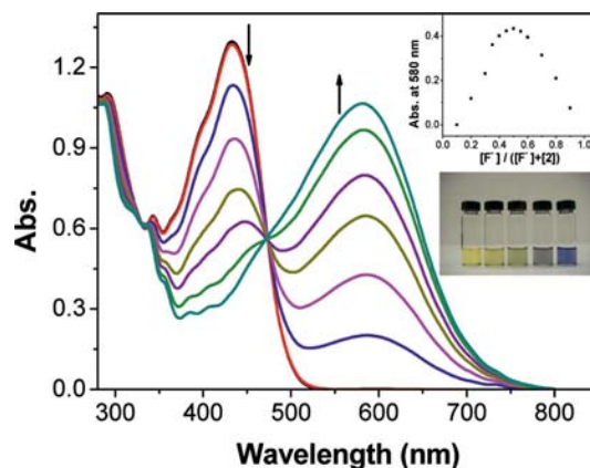
Figure 6. UV/Vis spectral changes of a DMSO solution of 2 ( 4.0 \times 10^{-5} \text{ mol L}^{-1} ) upon addition of a solution of (\text{Bu}_4\text{N})\text{F} ( 1.0 \times 10^{-2} \text{ mol L}^{-1} ). The inset shows the Job plot for the binding of 2 to \text{F}^- monitored at 580 nm ( [\text{F}^-] + [\text{2}] = 4.0 \times 10^{-5} \text{ mol L}^{-1} ) and the color change of DMSO solutions of 2 upon addition of (from left to right) 0, 0.25, 0.5, 0.75, and 1.0 equiv. \text{F}^- .
