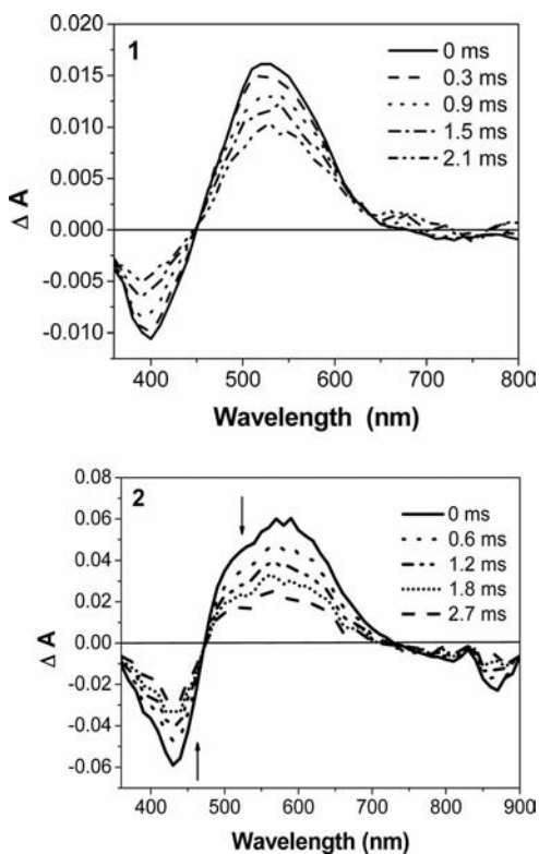
Figure 3. Time-resolved triplet transient difference absorption spectra of 1 and 2 in DMSO following excitation at 355 \text{ nm} . The concentration of the solutions was 4.0 \times 10^{-5} \text{ mol L}^{-1} .
