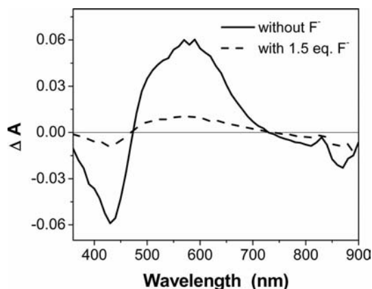
Figure 8. Triplet transient difference absorption spectra of 2 in 4.0 \times 10^{-5} \text{ mol L}^{-1} DMSO solutions without [\text{Bu}_4\text{N}]\text{F} and with 1.5 equiv. [\text{Bu}_4\text{N}]\text{F} immediately after the 355 \text{ nm} excitation.
