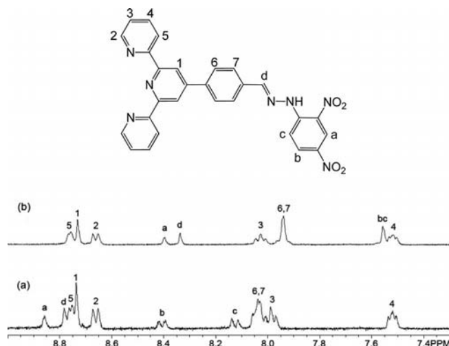
Figure 9. The downfield ^1\text{H} NMR (400 MHz) spectra of 1 in [\text{D}_6]\text{DMSO} at 25^\circ\text{C} without (\text{Bu}_4\text{N})\text{F} (a) and with excess (\text{Bu}_4\text{N})\text{F} (b).
