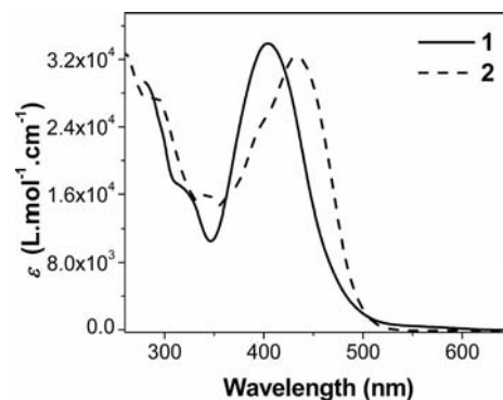
Figure 1. UV/Vis absorption spectra of 1 and 2 in DMSO solution.
