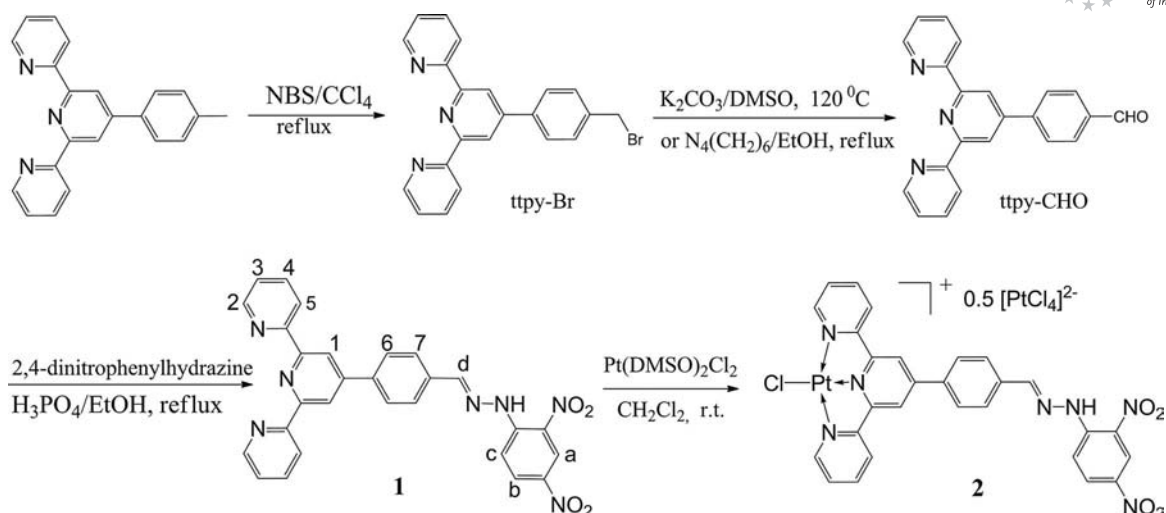
Scheme 1. Synthetic route and structures for 1 and 2 .
