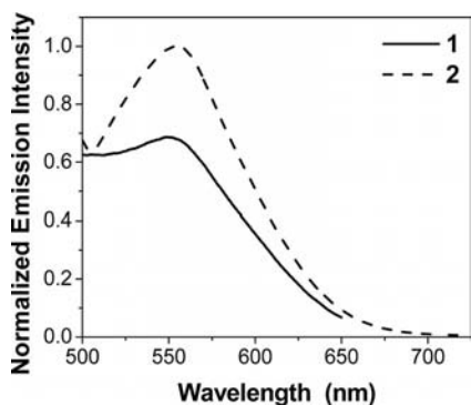
Figure 2. Normalized emission spectra of compounds 1 and 2 in DMSO at a concentration of 4.0 \times 10^{-5} \text{ mol L}^{-1} ( \lambda_{\text{ex}} = 404 \text{ nm} for 1 and 433 \text{ nm} for 2 ).
