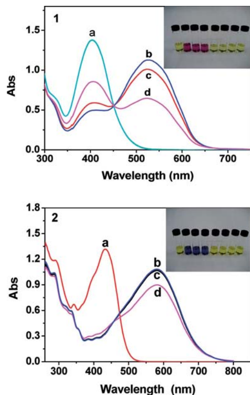
Figure 4. UV/Vis absorption spectra of 4.0 \times 10^{-5} \text{ mol L}^{-1} DMSO solutions of 1 (top) and 2 (bottom) after addition of 10 equiv. of either \text{Cl}^- , \text{Br}^- , \text{I}^- , \text{NO}_3^- , or \text{HSO}_4^- (a), 1 equiv. \text{F}^- (b), 1 equiv. \text{AcO}^- (c), or 1 equiv. \text{H}_2\text{PO}_4^- (d). Insets show the color pictures of the original solutions of 1 (top) and 2 (bottom) ( 4 \times 10^{-5} \text{ mol L}^{-1} ) and the solutions with different anions [from left to right: original solution, solutions with \text{F}^- (1 equiv.), \text{AcO}^- (1 equiv.), \text{H}_2\text{PO}_4^- (1 equiv.), \text{Cl}^- (10 equiv.), \text{Br}^- (10 equiv.), \text{I}^- (10 equiv.), and \text{NO}_3^- (10 equiv.)].
